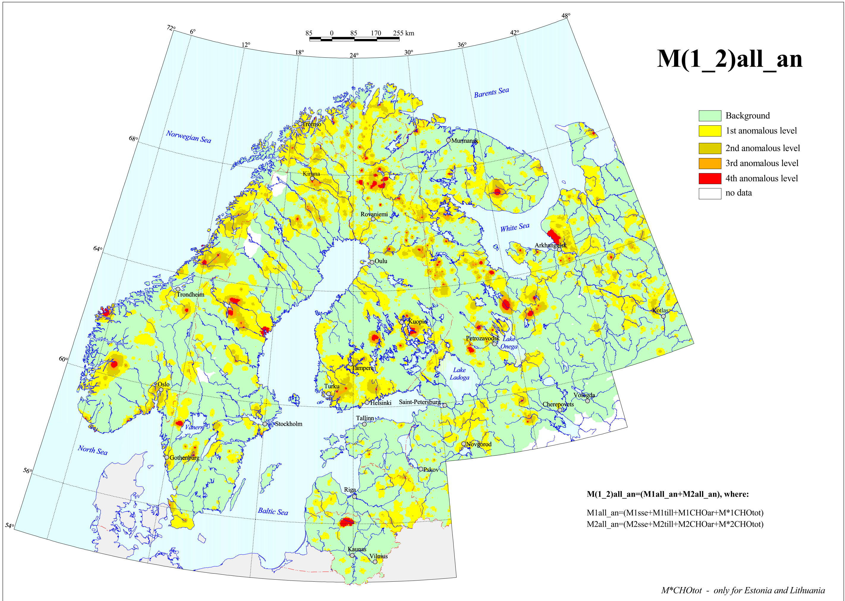
Integrated Anomalous Geochemical Fields, M(1_2)all_an
